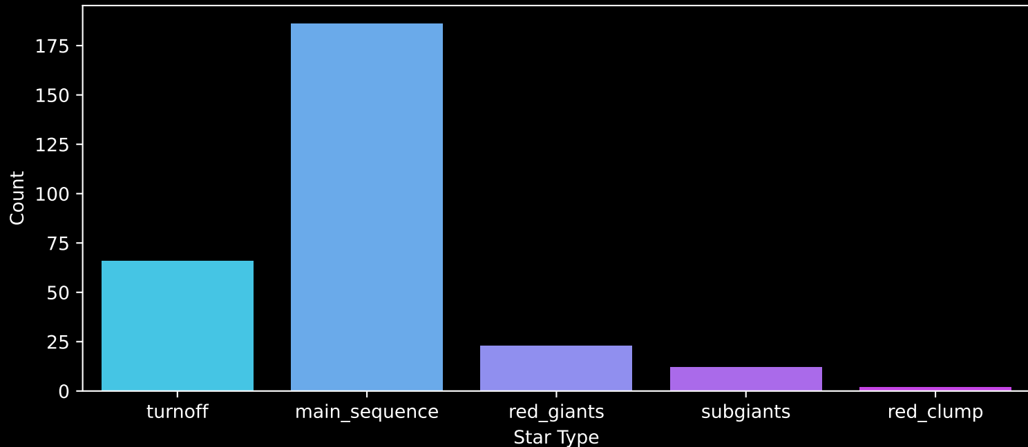
GALAH DR4 Field: [6951] Count plot of Star Type
