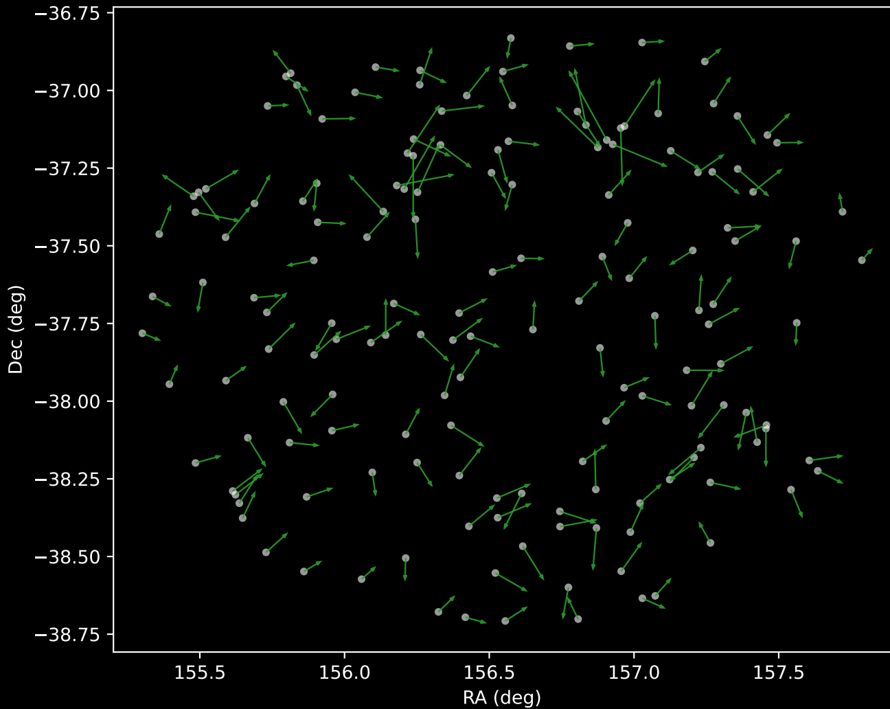
GALAH DR4 Cluster 4 Proper Motion Vectors (n=159)
