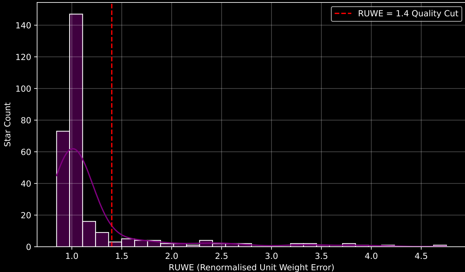
GALAH DR4 Field [6951] RUWE Distribution (n= 286)
