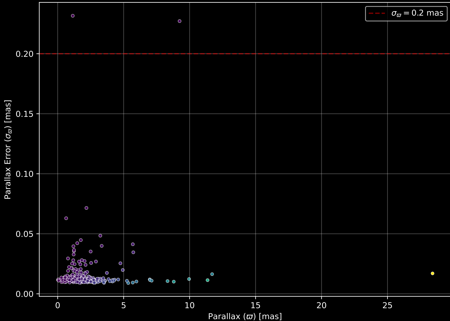
GALAH DR4 Field: [6951] Parallax Quality (n= 289)
