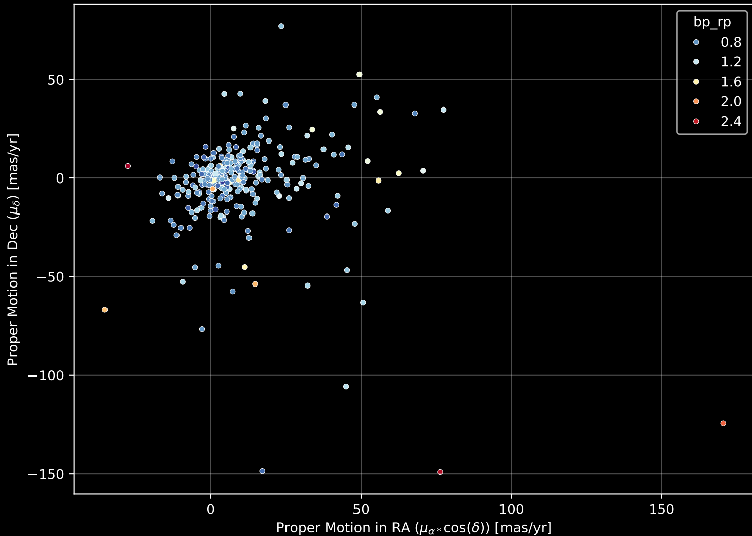
GALAH DR4 Field: [6951] Proper Motion Diagram (n= 289)
