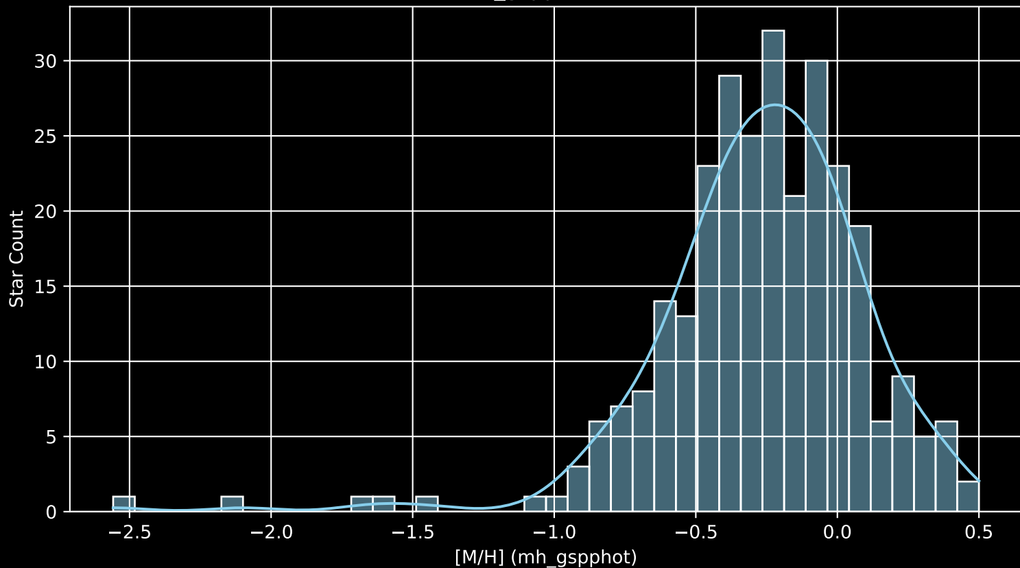
GALAH DR4 Field: [6951] [M/H] (mh_gspphot) (n= 288)
